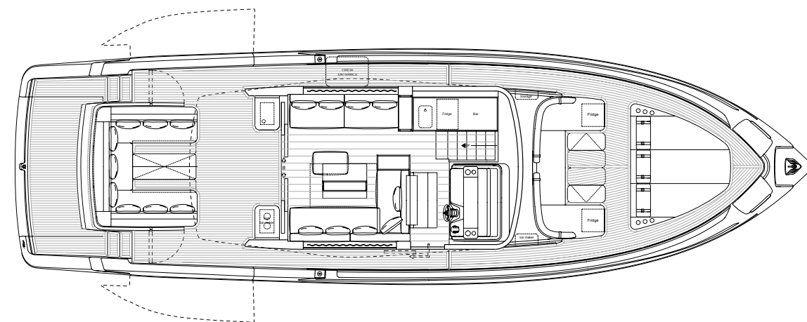
MAIN DECK - V2 LIVING VERSION
