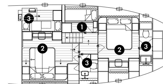
LOWER DECK - V2 CABIN VERSION
