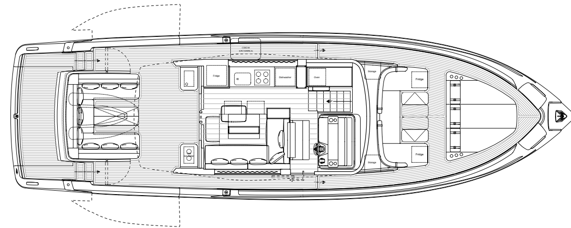
MAIN DECK - V1 KIKTCHEN VERSION
